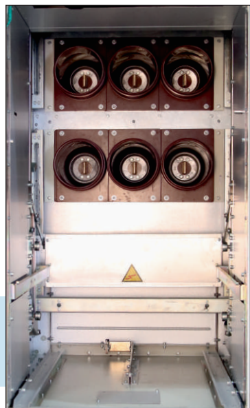
■ CB chamber with breaker removed and shutters open
